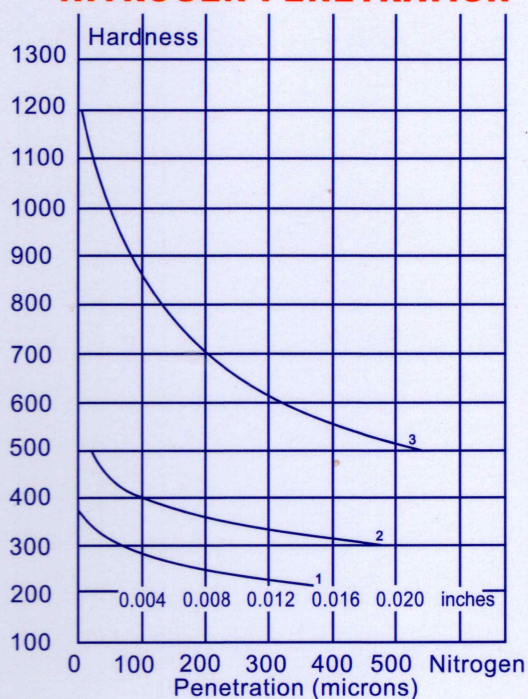
Figure 1 NITROGEN PENETRATION
